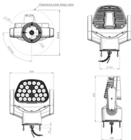
SL1 Measurement Drawing
